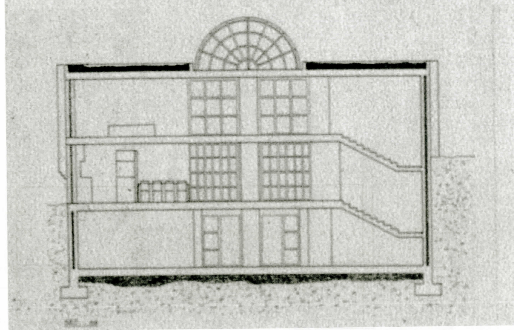
SECTION AA
